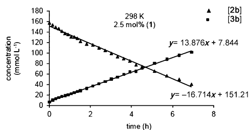
Figure 1. Kinetic profile of the CDC of 2b at 298 K in the presence of 2.5 mol % of 1 .
